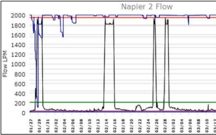
Figure 5 – Catchment 2 flow graph.
